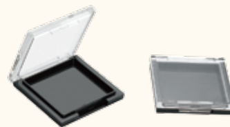
Item No: LB-306 L/W/H: 67.2*67.2*12mm Size of well: 54.37*54.37*5mm
