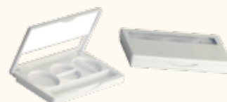
Item No: LB-516C L/W/H: 91.5*51*11.65mm Size of well: 24.13*16.13*5.31mm*3 /72.99*10.58*4.14mm
