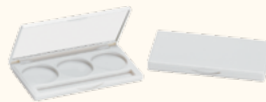
Item No: LB-922 L/W/H: 119.4*63.14*11.4mm Size of well: ø37*3.65mm*3 /108.15*14*4.25mm
