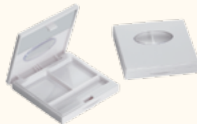
Item No: LB-103 L/W/H: 63.8*63.8*12.5mm Size of well: 33.15*27.7*4.75mm*2 /56.6*12.1*4.75mm
