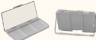
Item No: LB-A305A L/W/H: 87.0*54.8*6.8mm Size of well: 26.69*41.49*4.2mm*3
