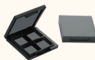
Item No: LB-307 L/W/H: 67.5*67.2*12mm Size of well: 26.05*26.05*5mm*4
