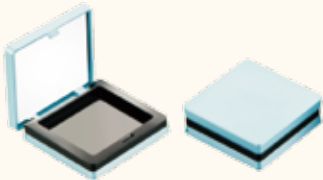
Item No: LB-A037B L/W/H: 55.32*55.32*15.23mm Size of well: 43.0*43.0*5mm
