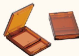
Item No: LB-302 L/W/H: 76.5*51.3*13.1mm Size of well: 43.3*43.3*5.5mm /43.3*20.4*5.5mm
