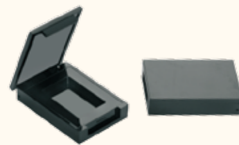
Item No: LB-401A L/W/H: 58.4*40.2*13.1mm Size of well: 48.1*35.9*7mm
