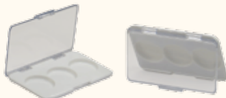
Item No: LB-A305 L/W/H: 87*54.8*6.9mm Size of well: ø27.2*4.2*3mm
